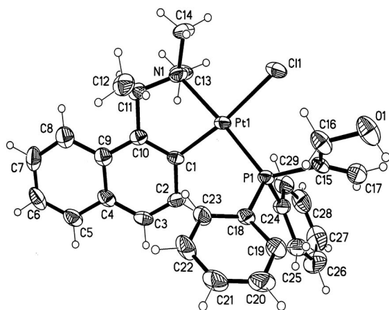
Figure 4. Molecular structure and absolute configuration of ( R C , S P )- 10 .
