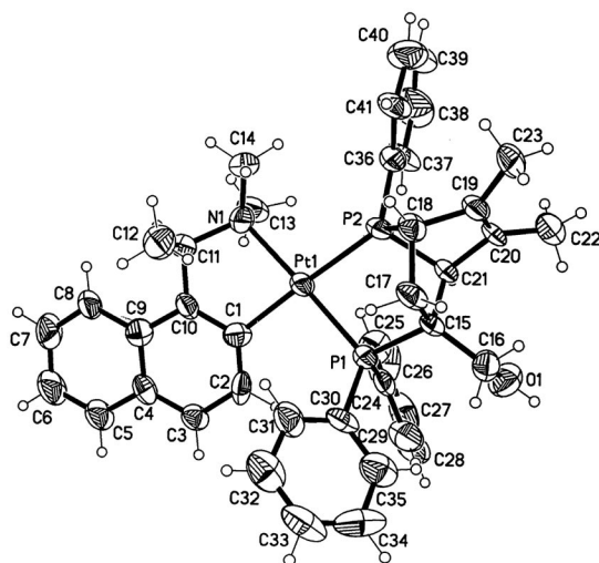
Figure 5. Molecular structure and absolute configuration of ( R C , S P )- 12 .
