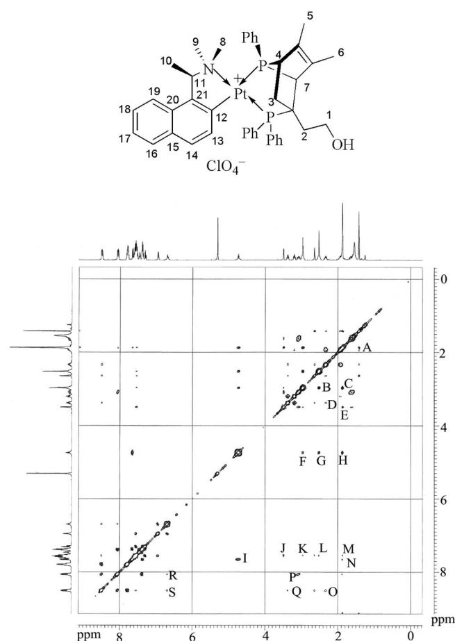
Figure 2. 500 MHz 2D ROESY spectrum of ( R C , S P )- 6 in CD 2 Cl 2 . Selected NOE interactions: (A) Me5–Me6; (B) NMe(eq)–NMe(ax); (C) Me10–NMe(eq); (D) H3–H4; (E) Me6–H7; (F) NMe(ax)–H11; (G) NMe(eq)–H11; (H) Me10–H11; (I) H11–H19; (J) H7–PPh; (K) NMe(ax)–PPh; (L) NMe(eq)–PPh; (M) Me10–PPh; (N) Me10–H19; (O) H3– o -Ph; (P) H7– o -Ph; (Q) H7– o -Ph'; (R) H13– o -Ph; (S) H13– o -Ph'.
