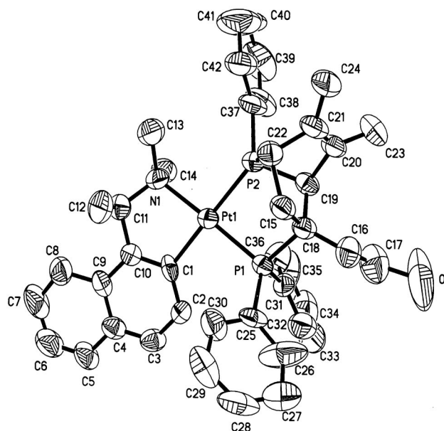
Figure 1. Molecular structure and absolute configuration of ( R C,S P )- 6 .
