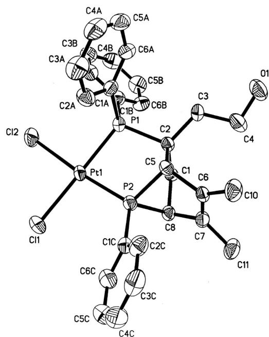
Figure 3. Molecular structure of ( S p )-7.
