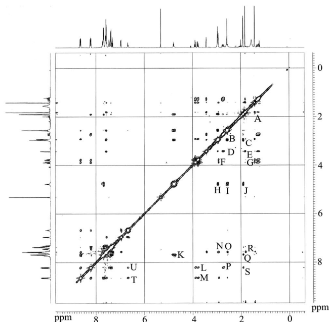
Figure 6. 500 MHz 2D ROESY spectrum of ( R C , S P )- 12 in CD 2 Cl 2 . Selected NOE interactions: (A) Me4–Me5; (B) NMe(eq)–NMe(ax); (C) Me9–NMe(eq); (D) H2–H1; (E) Me5–H1; (F) Me(ax)–H3; (G) Me4–H3; (H) Me(ax)–H10; (I) Me(eq)–H10; (J) Me9–H10; (K) H10–H18; (L) H6– o -Ph; (M) H6– o -Ph'; (N) NMe(ax)–PPh; (O) NMe(eq)–PPh; (P) H2– o -Ph'; (Q) Me9–PPh; (R) Me5–PPh; (S) Me9– o -Ph'; (T) H12– o -Ph'; (U) H12– o -Ph.
