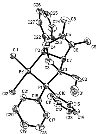
Figure 7. Molecular structure and absolute configuration of ( S P )- 13 .
